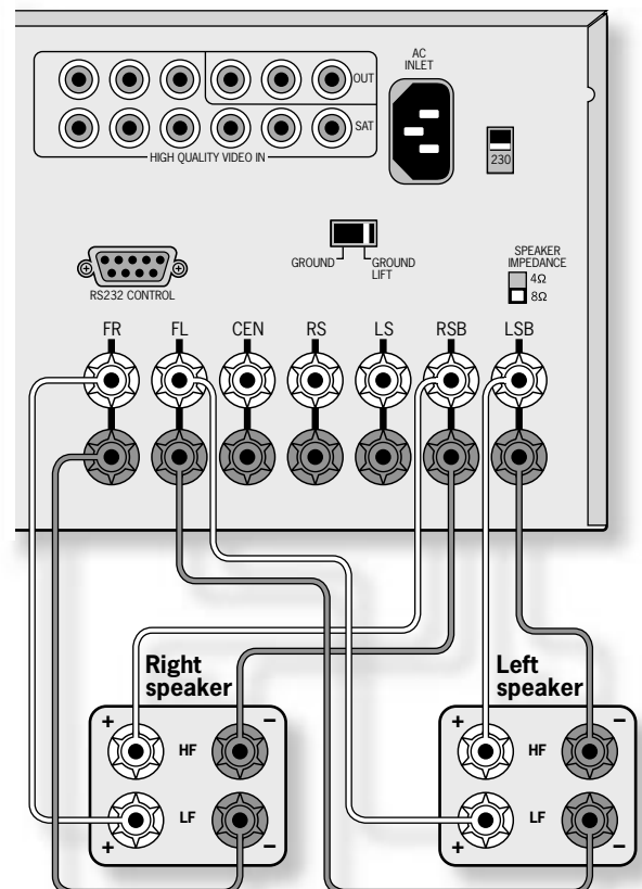
Bi-amping using the surround back channels of the AVR300 (only the front left and right speakers are shown, for clarity)
