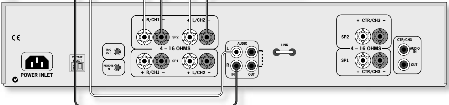
Bi-amping using the AVR300 and a P90 (only the front left and right channels are shown, for clarity)
