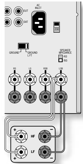
Bi-wiring using the AVR300 (only one speaker is shown, for clarity)
